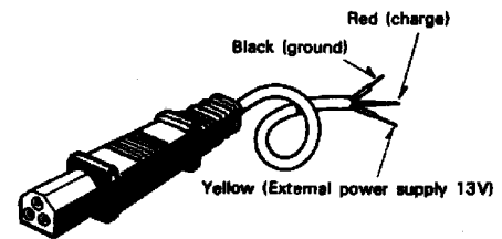
Fig. 8 Power Plug with Lead
