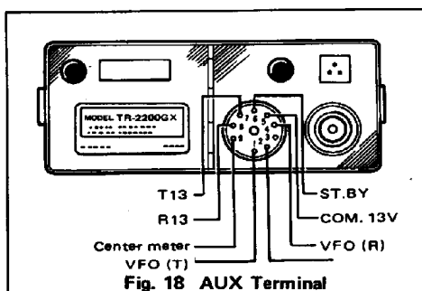
Fig. 18 AUX Terminal
